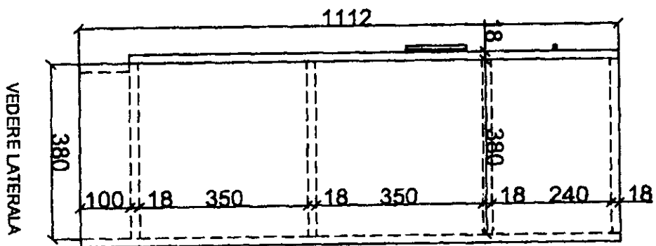
DULAP - CORP2 SCARA 1:10
