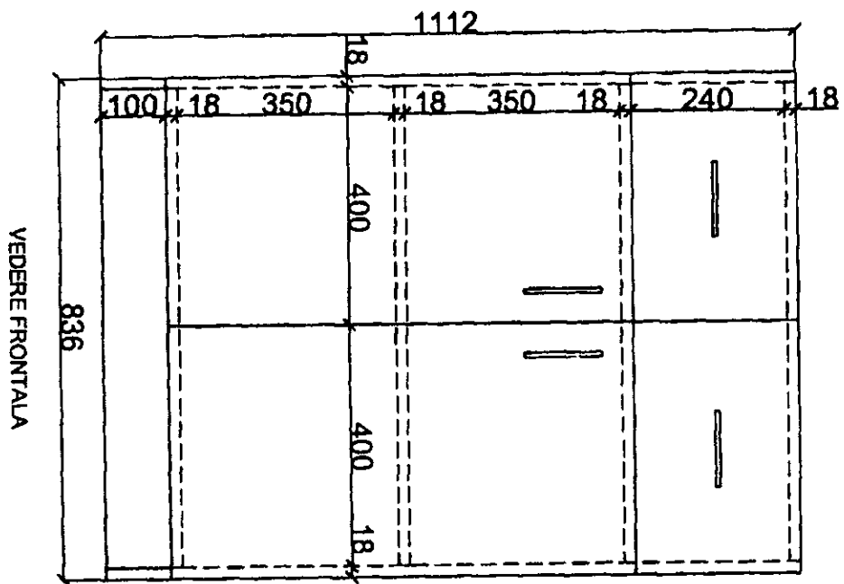
DULAP - CORP2 SCARA 1:10
